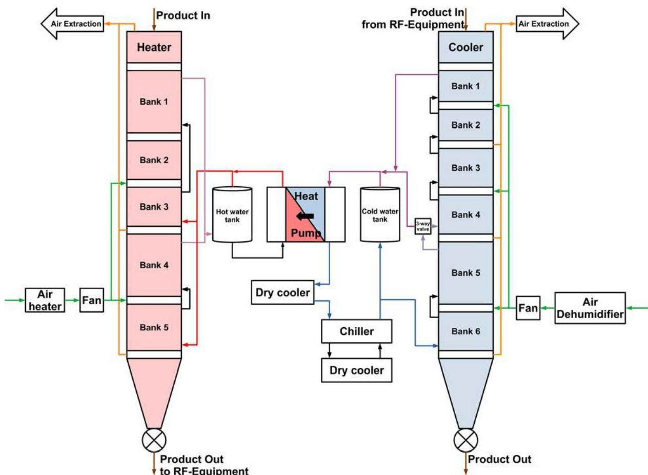
Schematic of the Solex moving bed heat exchangers, chiller, dry cooler and heat pump.
